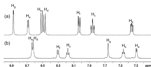
Figure 1. a) The aromatic region of the 1 H NMR spectrum of ligand (CD 2 Cl 2 , 400 MHz, 298 K) and b) of the cage 1 (CD 3 CN, 500 MHz, 298 K).
