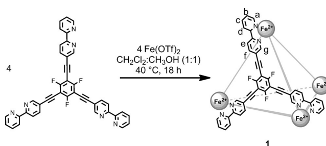
Scheme 1. Synthesis of [Fe 4 L 4 (OTf) 3 ] cage 1 ; only one ligand structure is shown for clarity.
