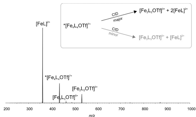
Figure 3. The ESI-QTOF CID spectrum for the isolated [Fe 4 L 4 (OTf)] 7+ ion (marked with a star) and its fragmentation pathway.
