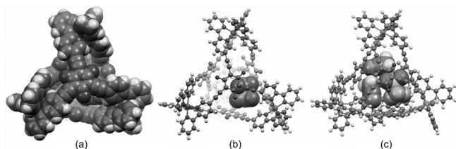
Figure 2. The crystal structure of 1 -ACN [only one cage, ΛΛΛΛ- 1 , is shown in (a) and (b)] and the molecular model of [(OTf − + 2ACN)C + ] 1 (c, SPARTAN, [14] MM level).
